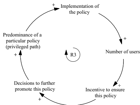
Figure 3. Balancing (B) and reinforcing (R) feedback loops identified in the QSDM. (a) Morphological equilibrium of the estuary – Loops B1, B2 and B3. (b) River engineering measures and sediment transport loops – R1 and R2. (c) Path dependency loop – R3. (d) Urban development loops – R4 and R5. (e) Car dependency loop – R6. (f) Risk awareness and “levee effect” loops – B4 and R7. (g) Poverty loop – R8. (h) Urban health and health-related damage loop – R9. (i) Urban health and income loop – R10. (j) Silo-thinking loop – R11.
